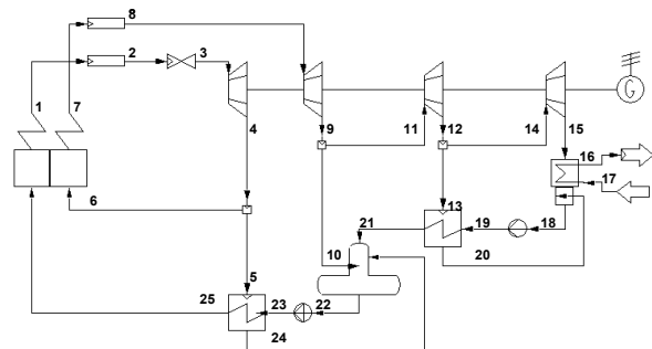
Figure 1. Design of steam cycle
