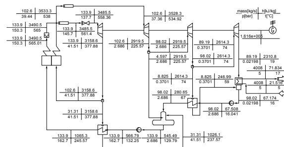
Figure 3. Simulation results in IPSEpro
